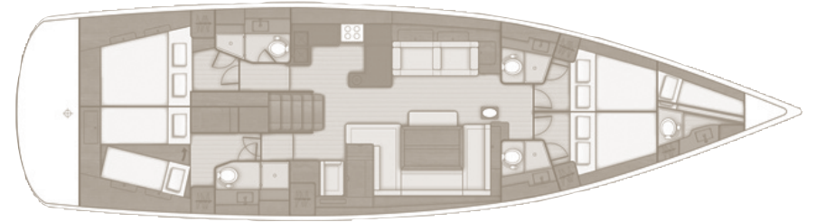
2 forward cabins - 2 head compartments, 2 Aft cabins 2 head compartments + Forepeak cabin (optional)
